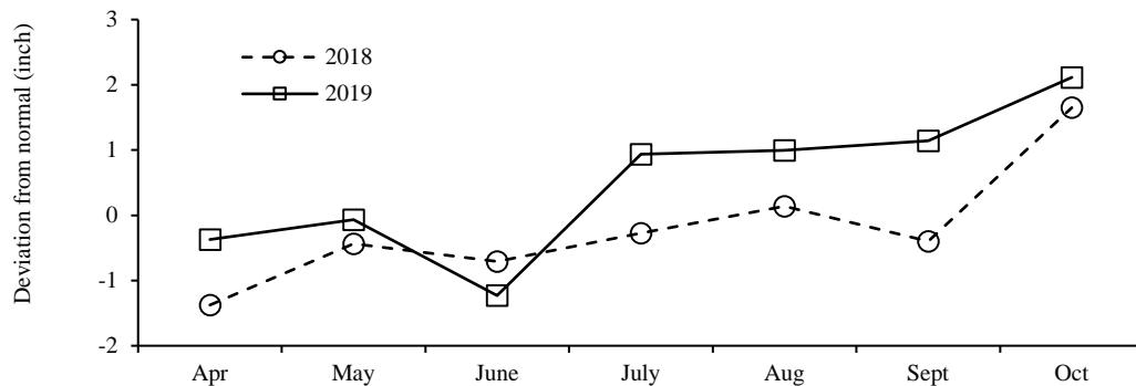
Figure 1: Deviation from normal precipitation (5 year average) during 2018 and 2019 at Ada, MN.
