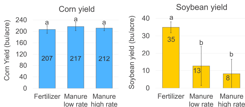
Figure 1. Corn (adjusted to 15.5% moisture) and soybean (adjusted to 13% moisture) yield at Murdock site in 2020. Manure was fall applied at 14,400 gallons per acre (high rate) or 9,500 gallons per acre (low rate) and fertilizer was spring applied. Different letters above a bar within a graph indicate a significant difference ( P < 0.05 ).
